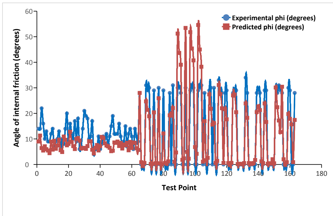
Fig. 4. Experimental Test Results for experimental and predicted ( \phi )
