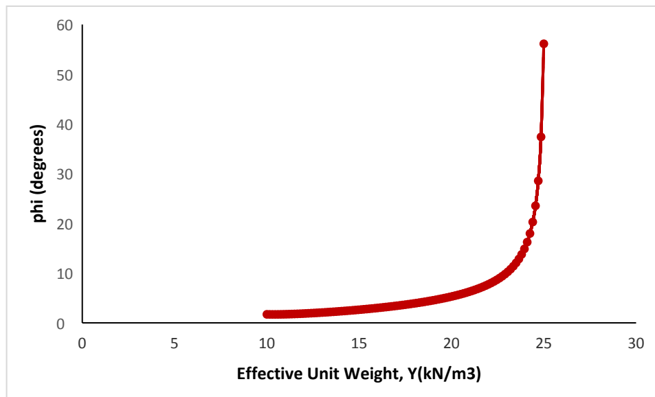
Fig. 12. Prediction of angle of internal friction with increase in effective unit weight ( \gamma )
