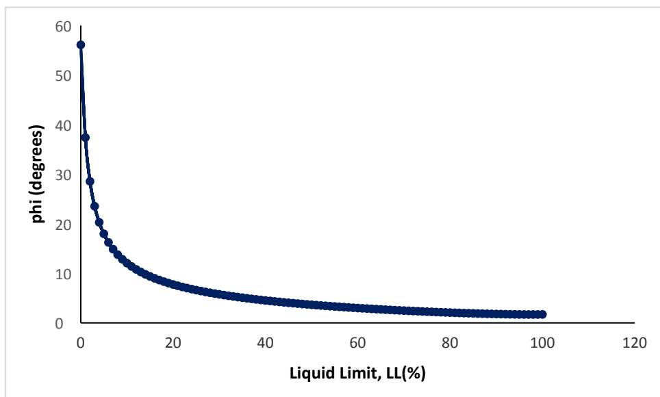
Fig. 8. Prediction of angle of internal friction with decrease in liquid limit (LL)
