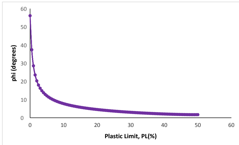
Fig. 10. Prediction of angle of internal friction with decrease in plastic limit (PL)
