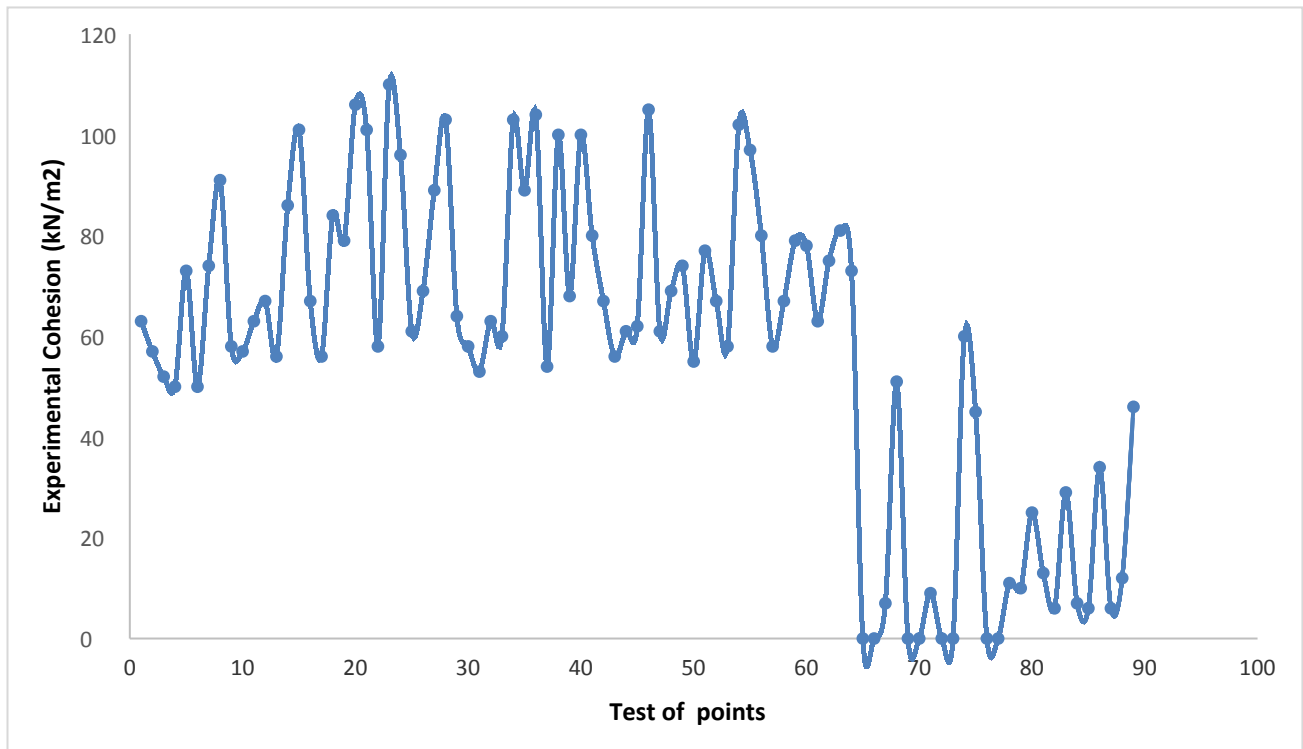
Fig. 2. Experimental Test Results for Cohesion ( C_u )
