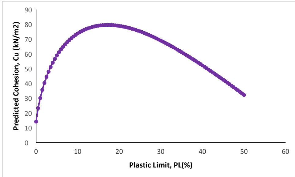
Fig. 9. Prediction of cohesion with decrease in plastic limit (PL)
