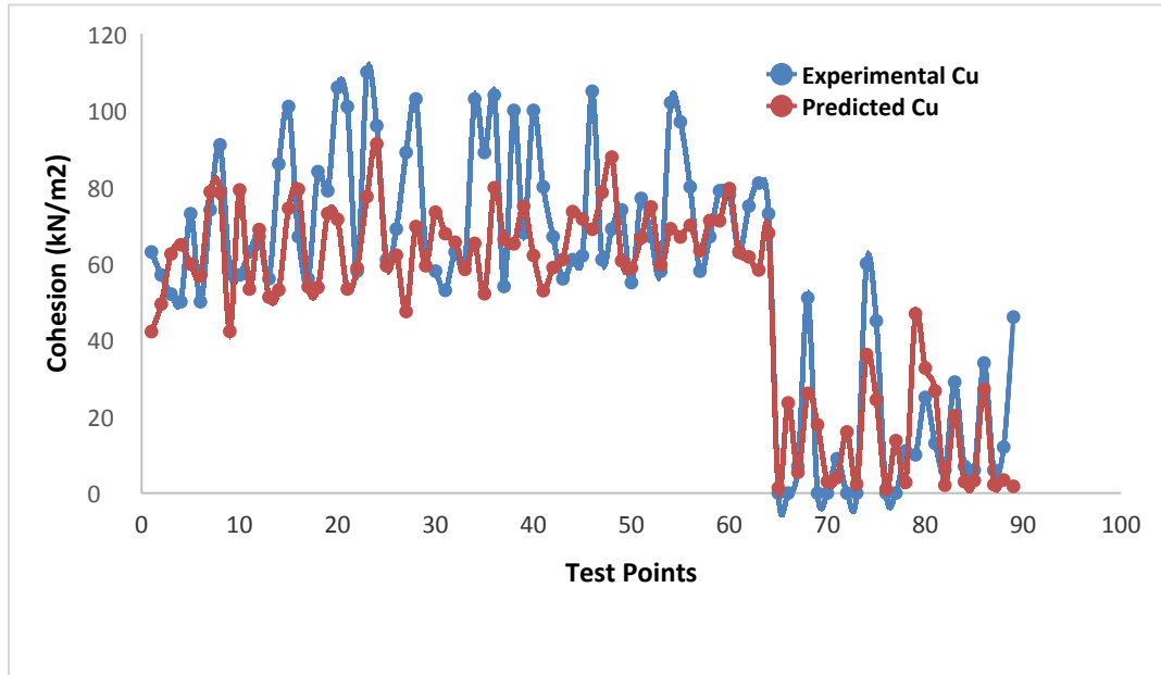
Fig. 3. Experimental Test Results for Experimental and Predicted (Cu)
