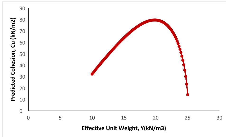
Fig. 11. Prediction of cohesion with increase in effective unit weight ( \gamma )
