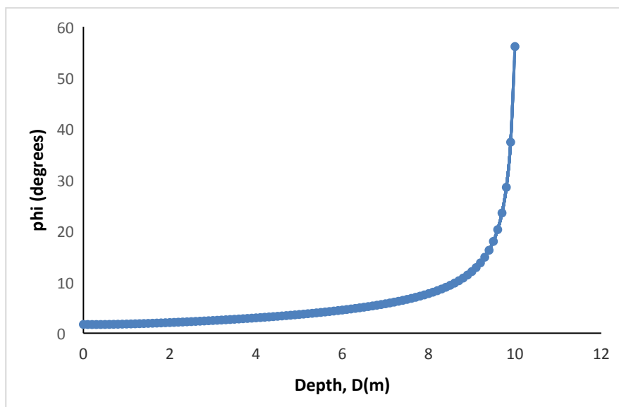
Fig.6. Prediction of angle of internal friction with increase in depth (d)
