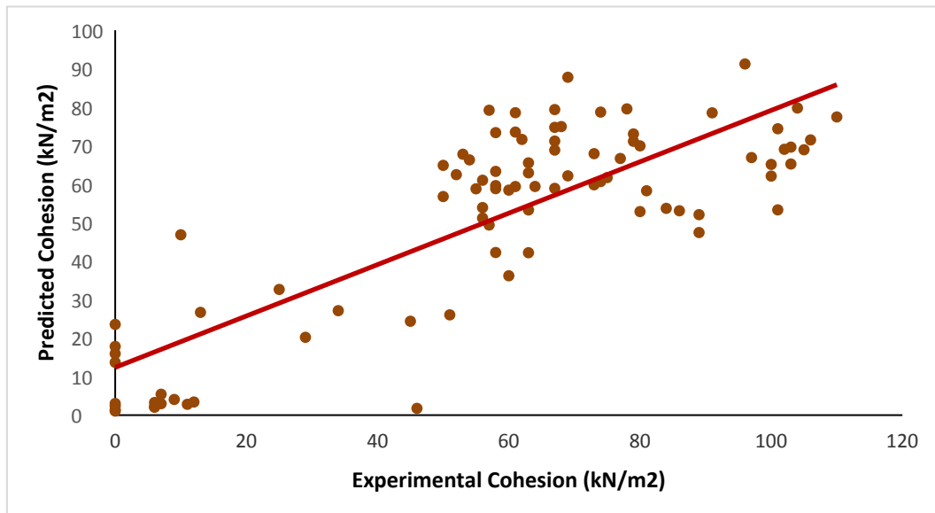
Fig. 13. Correlation coefficient of the experimental and predicted cohesion ( C_u )
