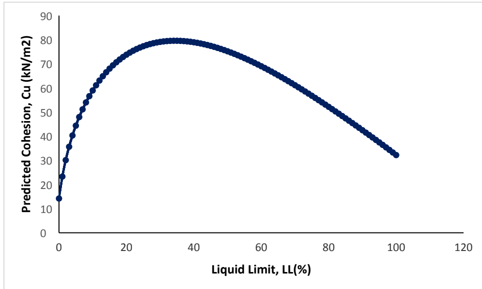
Fig.7. Prediction of cohesion with decrease in liquid limit (LL)
