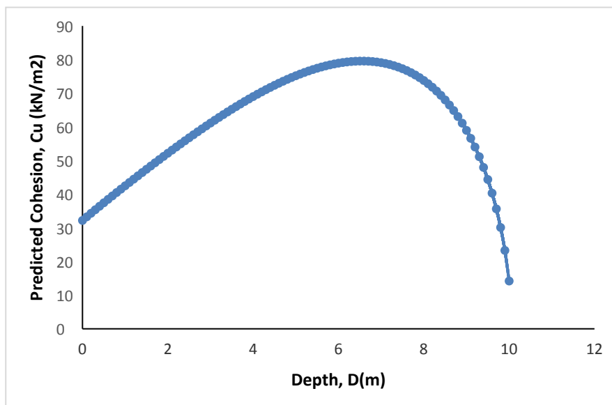
Fig. 5. Prediction of cohesion with increase in depth (d)
