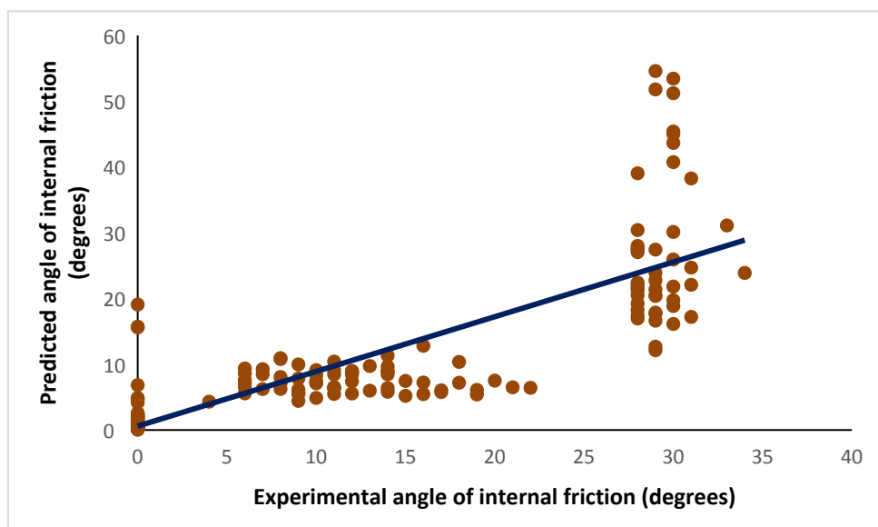
Fig. 14. Correlation coefficient of the experimental and Internal Friction
