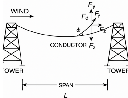
Figure 2 Sagging transmission line span between two towers showing wind velocity from left, drag force parallel to wind, lift force perpendicular to wind, and resolution into transverse component F_y along the sagging conductor (at sag angle \phi ) and vertical component. The span length is marked at the bottom.
