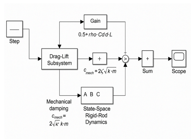
Fig 1 Simulink representation of the transmission lines
