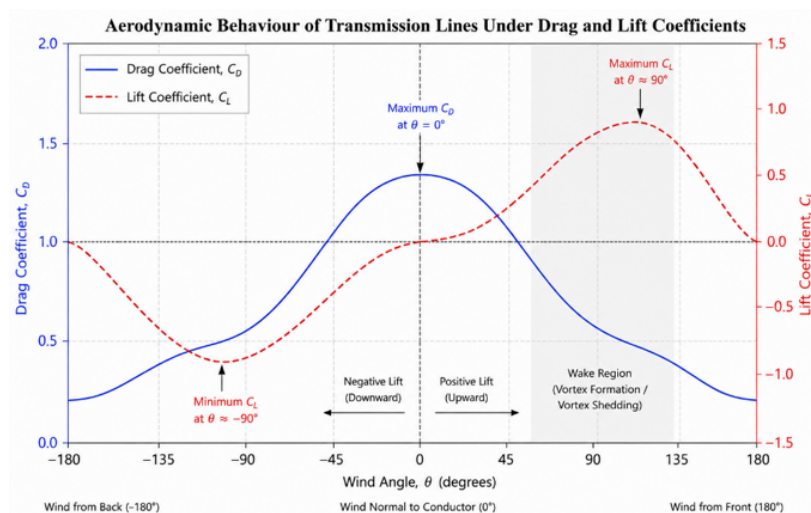
Fig 3: Aerodynamic Behaviour of Transmission Lines Under Drag and Lift Coefficients
