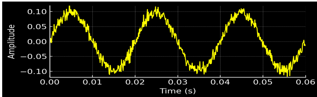
Figure 4 Simulated Mid-Span Displacement of ACSR 330 Conductor under Quasi-Steady Aerodynamic Damping
